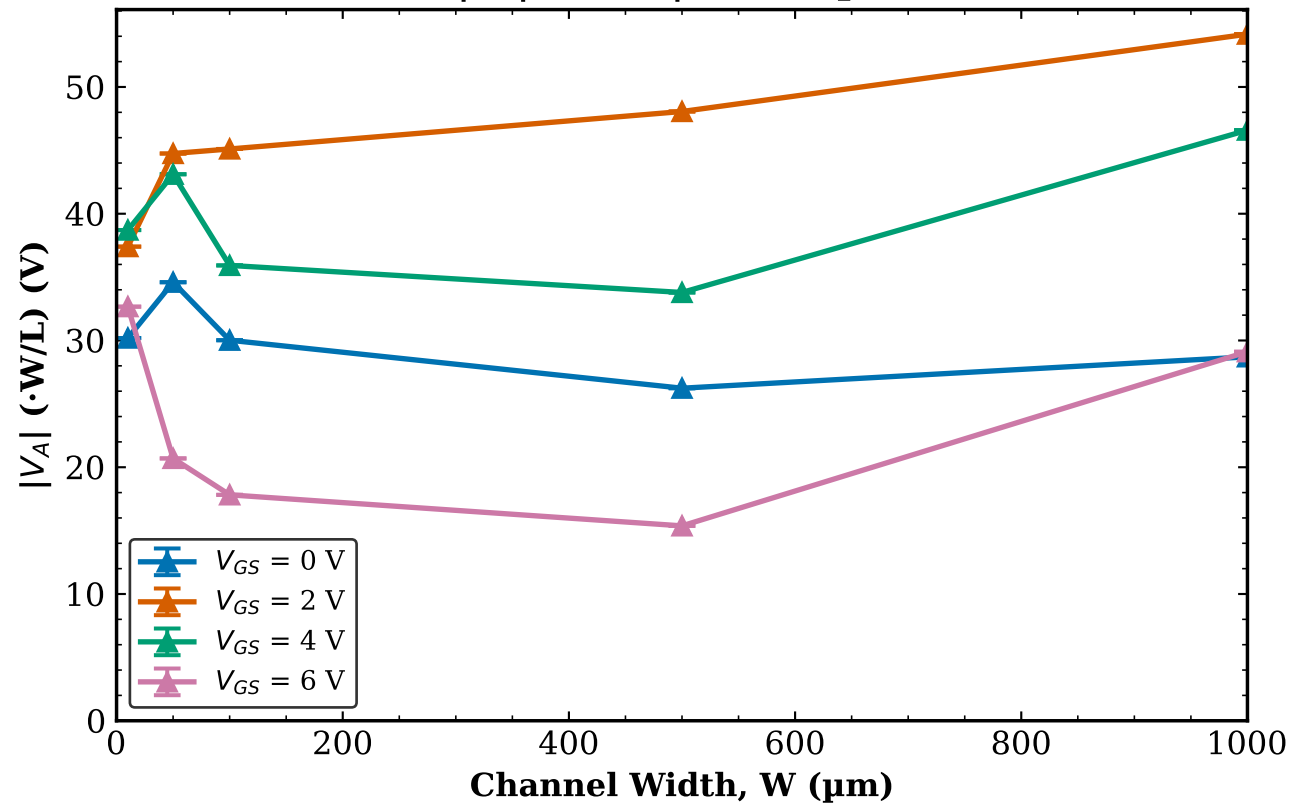
TFT1 Transistor 1 |V_A| vs W | L = 8\text{ }\mu\text{m}
